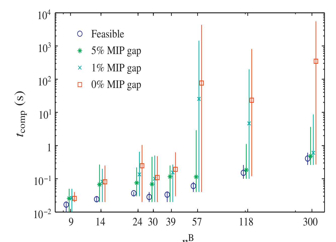
Figure 4: Mean, Max and Min times of Islanding Solutions
