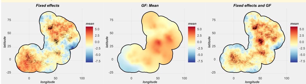
Contributions to the linear predictor
