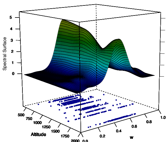
Figure 6. Spectral surface estimate using the double kernel estimator in (11); pseudo-angles are overlaid on the bottom of the box.
