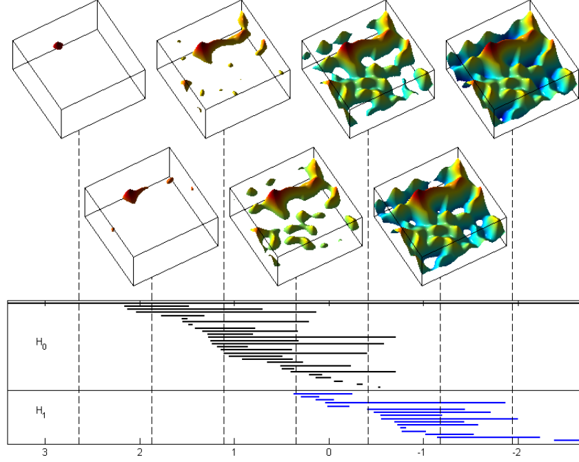
FIG 2.1. Barcodes for the excursion sets of a function on [0, 1]^2 . The top seven boxes show the surfaces generated by a 2-dimensional random field above excursion sets A_u for different levels u . To determine the level for each figure, follow the dotted line down to the scale at the bottom of the barcode. As the dotted lines pass through the boxes labelled H_0 and H_1 , the number of intersections with bars in the H_0 ( H_1 ) box gives the number of connected components (resp. holes) in A_u . Thus, at u \sim 1.9 , A_u has 4 connected components but no holes, while at u \sim -1.2 , A_u has only 1 connected component, but 9 holes. The horizontal lengths of the bars indicate how long the different topological structures (generators of the homology groups) persist. Computation of the barcodes was carried out in Matlab using the Plex (Persistent Homology Computations) from Stanford [11].
