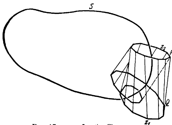
FIG. 17. z_1 \sim 2z_2 (in G ).
