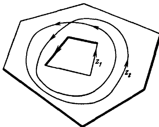
FIG. 14. z_2 \sim 2z_1 (in K ).
