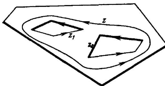
FIG. 13. z \sim z_1 + z_2 (in K ).
