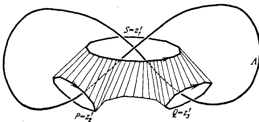
FIG. 16. z_1 \sim z_2 + z_3 (in G ).
