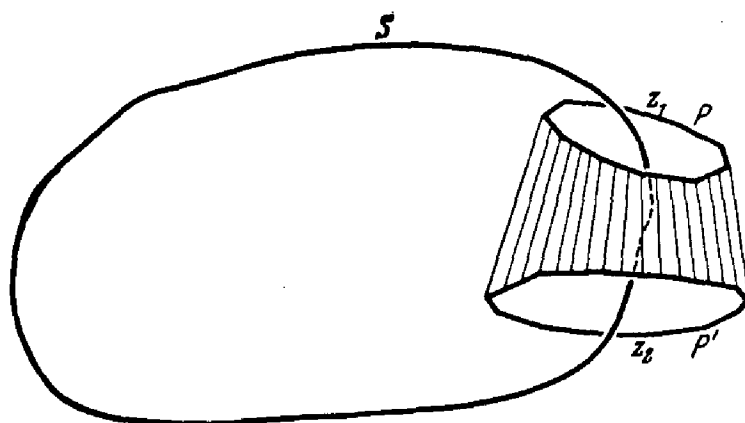
FIG. 15. z_1 \sim z_2 (in G ).
