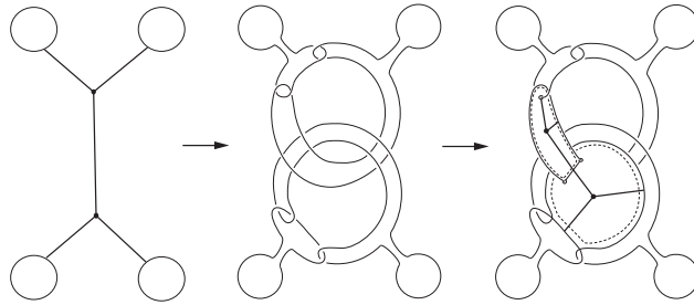
FIGURE 8. Realizing an order 2 tree in a Whitney tower by Bing doubling.
