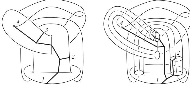
FIGURE 5. Both sides of this figure correspond to the slice of B^4 shown in the right-hand side of Figure 4. The tree t_p = \langle ((1, 2), 3), 4 \rangle is shown as a subset of the order 2 Whitney tower \mathcal{W} on the left. Replacing this left-hand side by the right-hand side illustrates the tree-preserving construction of a class 3 capped grope G^c bounded by L . In this case, the component G_1^c bounded by L_1 is the class 3 capped grope shown (partly translucent) on the right (together with a collar on L_1 ) which is gotten by surgering D_1 and W_{(1,2)} . The three other components of G are just the disks D_2 , D_3 and D_4 of \mathcal{W} , each of which has a single intersection with a cap of G_1^c .
