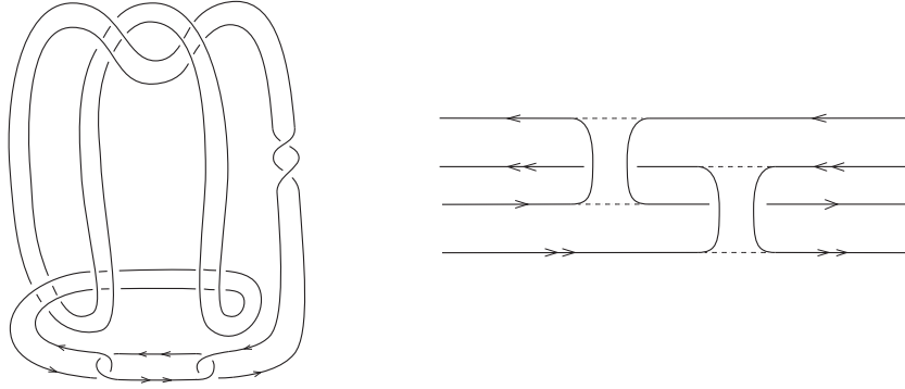
FIGURE 17. On the left, the (untwisted) Bing double of the figure-eight knot. On the right, disjoint Seifert surfaces for the two components of an untwisted Bing doubled knot can be constructed from four copies of a Seifert surface bounded by the original knot.
