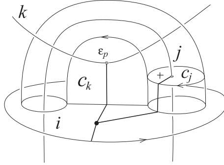
FIGURE 10. Near the trivalent vertex of the signed Y-tree \epsilon_p \cdot t_p = \epsilon_p \cdot \langle (i, j), k \rangle in a dyadic class 2 capped grope component (capped surface) bounded by L_i .
