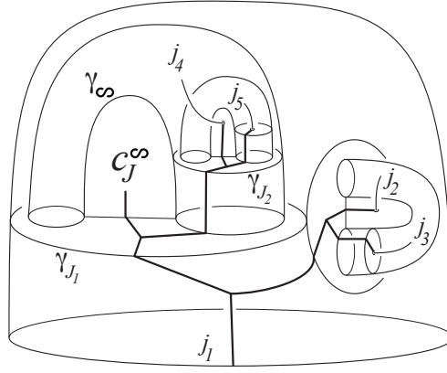
FIGURE 15. An example of Figure 14 with J_1 = (j_1, (j_2, j_3)) of order 2, and J_2 = (j_4, j_5) of order 1.
