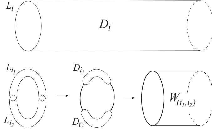
FIGURE 18. Pushing into B^4 from left to right: Above, a collar of L_i in D_i . Below, D_i yields a Whitney disk W_{(i_1, i_2)} for the intersections between D_{i_1} and D_{i_2} bounded by L_{i_1} and L_{i_2} , the untwisted Bing-double of L_i . D_{i_1} and D_{i_2} are traced out by null-homotopies of L_{i_1} and L_{i_2} ; and the curved vertical arcs are part of W_{(i_1, i_2)} .
