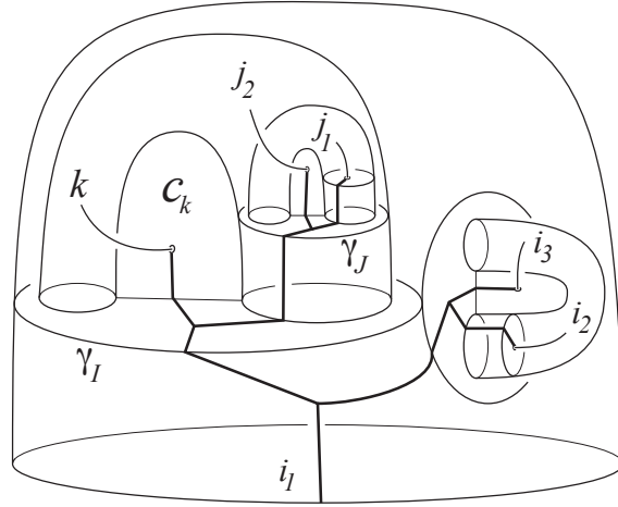
FIGURE 13. An example of Figure 12 with I = (i_1, (i_2, i_3)) of order 2, J = (j_1, j_2) of order 1, and K = k of order zero.
