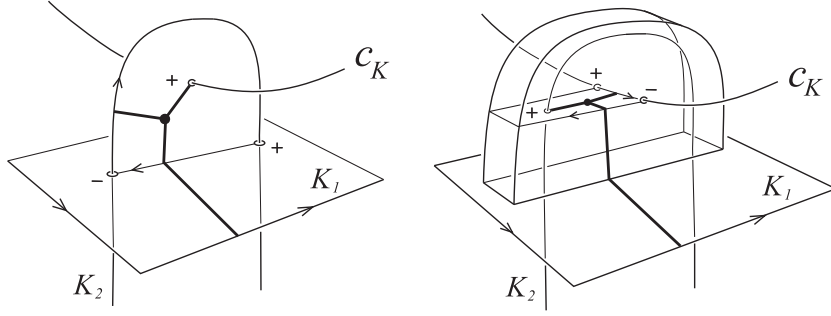
FIGURE 8. A Whitney move preserves the sign and orientation at a trivalent vertex.
