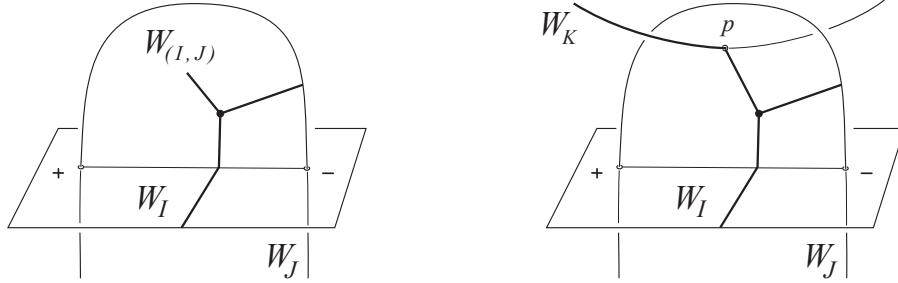
FIGURE 2. On the left, (part of) the rooted tree (I, J) associated to a Whitney disk W_{(I,J)} . On the right, (part of) the unrooted tree t_p = \langle (I, J), K \rangle associated to an intersection p \in W_{(I,J)} \cap W_K . Note that p corresponds to where the roots of (I, J) and K are identified to a (non-vertex) point in \langle (I, J), K \rangle .
