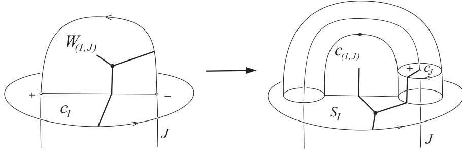
FIGURE 6. A surgery step in the resolution of an order n twisted Whitney tower to a class n+1 twisted capped grope. Any interior intersections in W_{(I,J)} and c_{(I,J)} are not shown.
