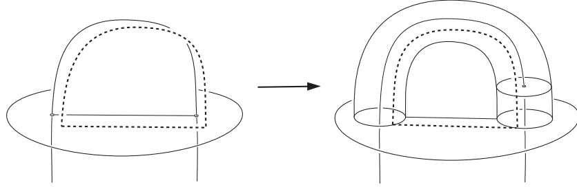
FIGURE 7. The framing obstruction determined by the Whitney section over the boundary of a Whitney disk is passed on to the framing obstruction on the cap resulting from surgery.
