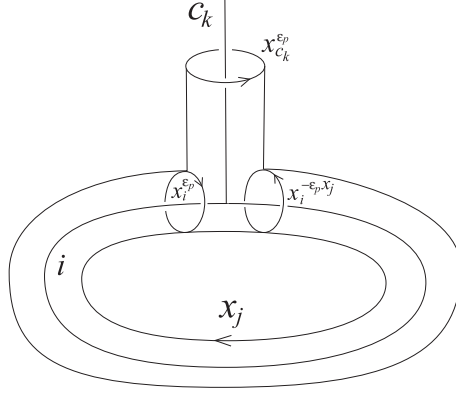
FIGURE 11. A meridian to the cap c_k in Figure 10 bounds a genus one surface which is a punctured normal torus to the surface stage containing the cap boundary. This normal torus consists of circle fibers in the normal circle bundle over a dual circle to the cap boundary in the surface stage. This dual circle is parallel to the boundary of the dual cap (which in Figure 10 represents the meridian x_j ). Since the (closed) normal torus has a single intersection with the cap it is also called a “dual torus” for the cap.
