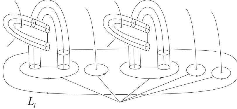
FIGURE 9. A parallel push-off of L_i is isotopic to a product of loops which are boundary circles of parallel push-offs of dyadic branches of G_i , or meridional circles to framed caps of G^c . So the corresponding factors \gamma_{i_r} of the i th longitude \gamma_i = \prod_r \gamma_{i_r} are in one-to-one correspondence with the i -labeled vertices of the trees in t(G^c) .
