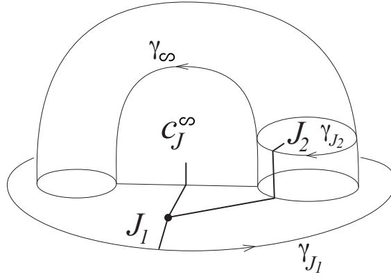
FIGURE 14. Near a twisted cap in a dyadic branch of G^c .
