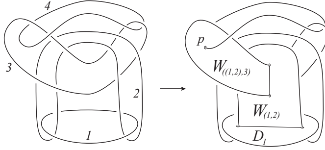
FIGURE 4. Pushing into B^4 from left to right, a Bing-doubled Hopf link L \subset S^3 bounds an order 2 Whitney tower \mathcal{W} : The order 1 disk D_1 consists of a collar on L_1 together with the indicated embedded disk on the right. The other three order 1 disks in \mathcal{W} consist of collars on the other link components which extend further into B^4 and are capped off by disjointly embedded disks. The Whitney disk W_{(1,2)} pairs D_1 \cap D_2 , and W_{((1,2),3)} pairs W_{(1,2)} \cap D_3 , with p = W_{((1,2),3)} \cap D_4 the only unpaired intersection point in \mathcal{W} .
