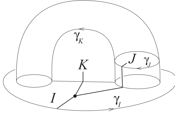
FIGURE 12. Near a trivalent vertex in a dyadic branch of G^c .
