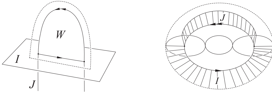
FIGURE 3. The Whitney section over the boundary of a framed Whitney disk is indicated by the dotted loop shown on the left for a clean Whitney disk W in a 3-dimensional slice of 4-space. On the right is shown an embedding into 3-space of the normal disk-bundle over \partial W , indicating how the Whitney section determines a well-defined nowhere vanishing section which lies in the I -sheet and avoids the J -sheet.
