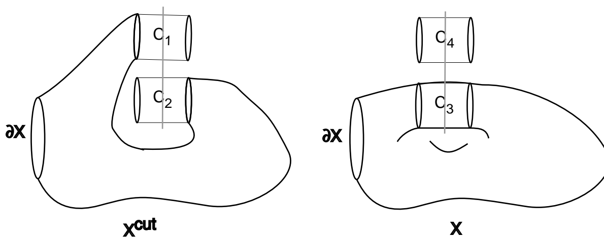
Figure 3: The map U
