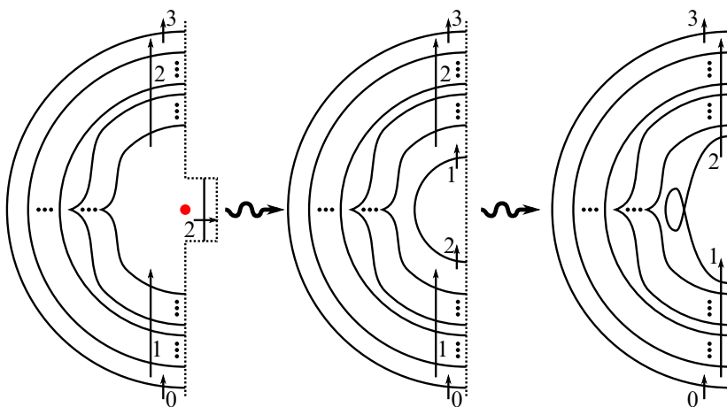
Figure 20: G_1 after attaching a 4–dimensional 2–handle
