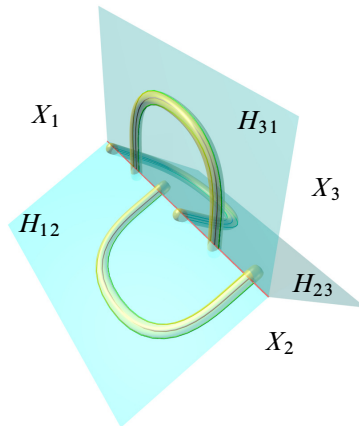
Figure 2: Stabilizing a trisection in dimension 3
