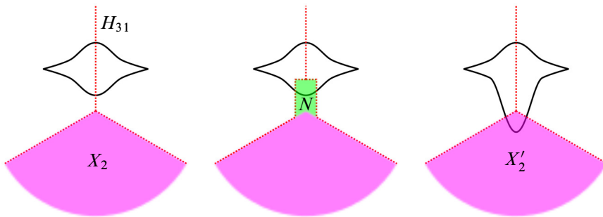
Figure 28: Adding one eye to a trisected Morse 2–function
