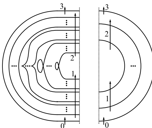
Figure 21: Two halves of G_1 : the 0-, 1- and 2-handles on the left and the 3- and 4-handles on the right. Connecting them with a Cerf graphic gives Figure 14.
