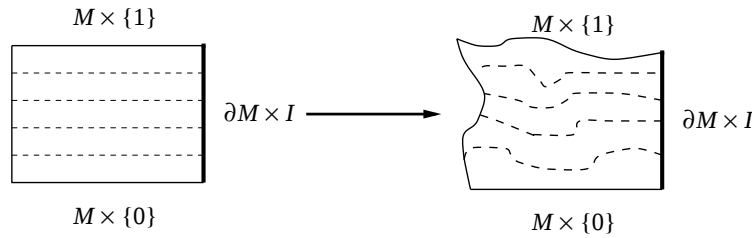
Fig. 3. A pseudo-isotopy
