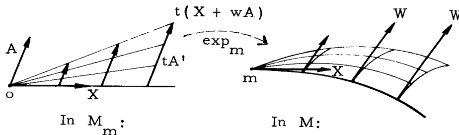
Fig. 10.1 Jacobi Field
