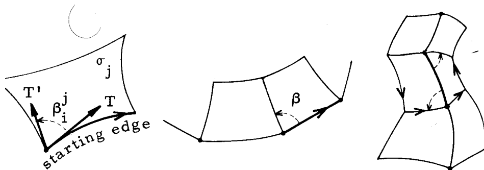
Fig. 8.4 Starting Edges
