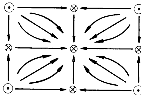
Fig. 8.6 The Canonical Vector Field on a 2-cube
