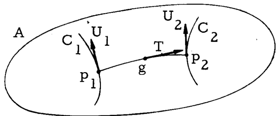
Fig. 10.4 Cross Manifolds
