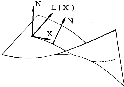
Fig. 2.1 The Weingarten Map (derivative of normal)
