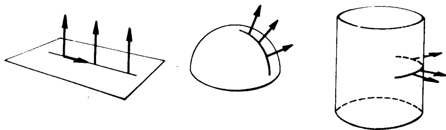
Fig. 2.3 Pieces of Examples (1), (2), (3)
