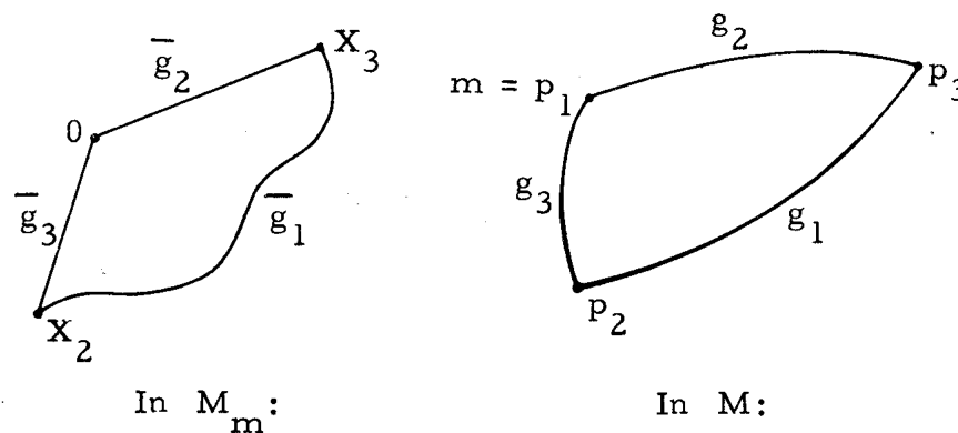
Fig. 10.6 Geodesic Triangle
