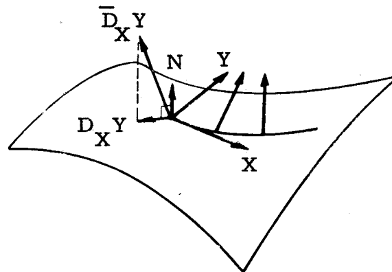
Fig. 2.2 Decomposition of \bar{D}_X Y
