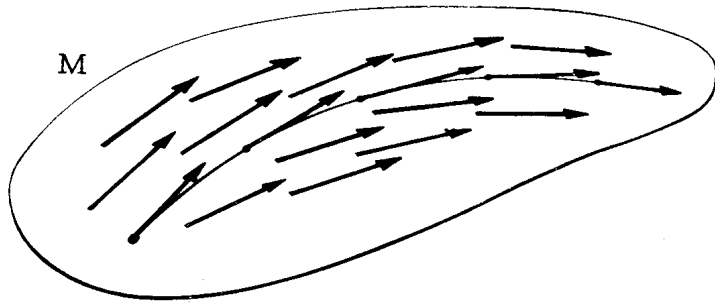
Fig. 1.4 An Integral Curve of a Vector Field
