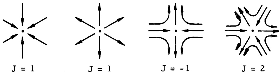
Fig. 8.5 Examples of J(W, m)
