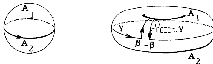
Fig. 8.3 Sphere and Torus
