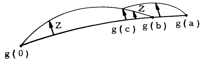
Fig. 10.2 Fields Along a Geodesic
