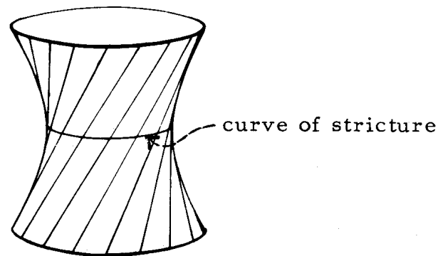
Fig. 2.6 Hyperboloid of Revolution
