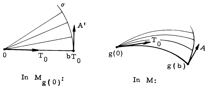
Fig. 10.3 Comparing Geodesics
