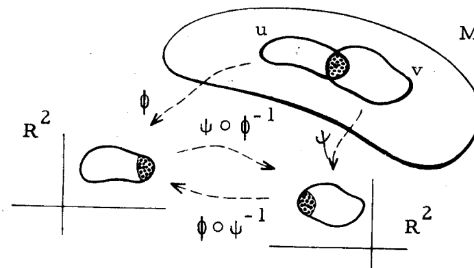
Fig. 1.1 Overlapping Coordinate Domains
