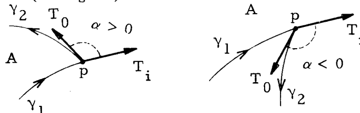
Fig. 8.1 Corner Angles
