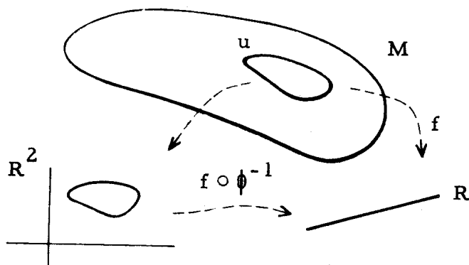
Fig. 1.2 An Induced Map from R^2 into R
