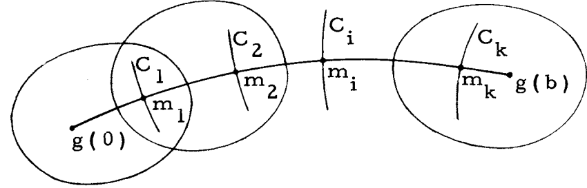
Fig. 10.5 Cross Manifolds
