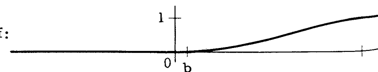
Fig. 6.1 Constructing a C^\infty Step Function
