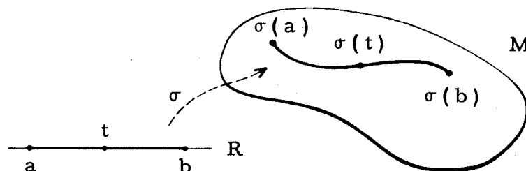
Fig. 1.3 A Curve
