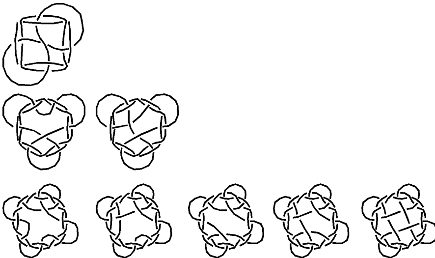
Fig. 5. Another series of Borromean links derived from the same source.
