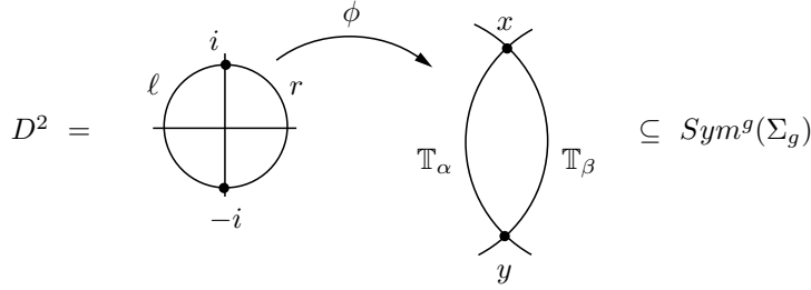
FIGURE 1. A Whitney disk.
