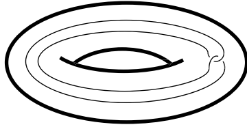
FIGURE 4. The satellite for the Whitehead double.
