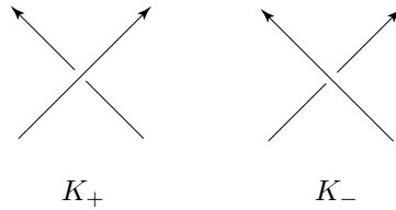
FIGURE 3. The knots K_+ and K_- differ only in the sign of one crossing.
