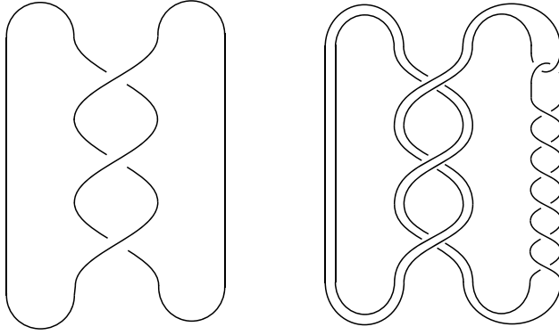
FIGURE 5. The untwisted Whitehead double of the right-handed trefoil. The 6 half-twists on the right have been added to ensure that the linking number is zero.
