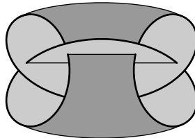
Figure 1.2: A ribbon disk
