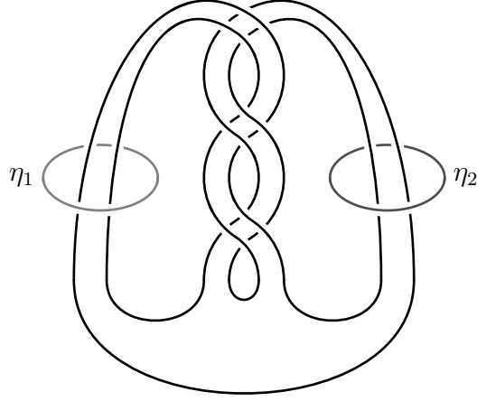
Figure 2.6: Paths along which 9_{46} is infected to yield J(K)
