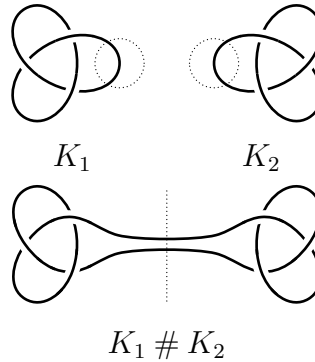
Figure 1.3: Connected sum in S^3
