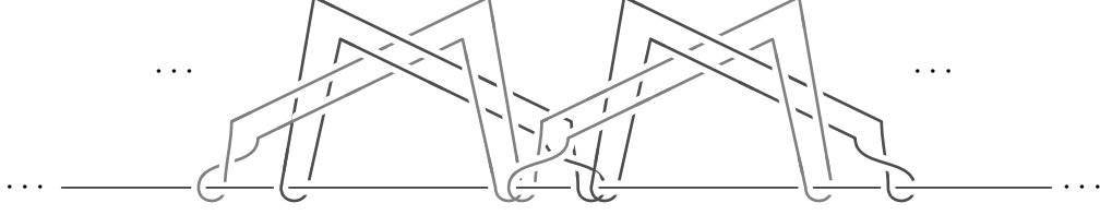
Figure 5.3: The infinite cyclic cover of (S^3, 9_{46})
