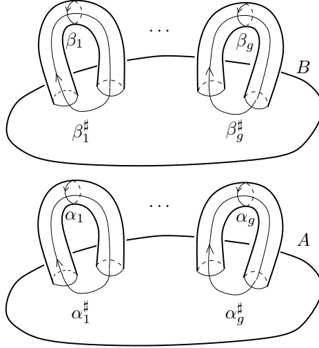
FIGURE 4.1. The curves \alpha, \alpha^\# on \partial A and the curves \beta, \beta^\# on \partial B .
