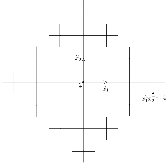
FIGURE A.1. The infinite tree \tilde{X}_2 , where x_1 acts by “horizontal translation” to the right and x_2 acts by “vertical translation” to the top.
