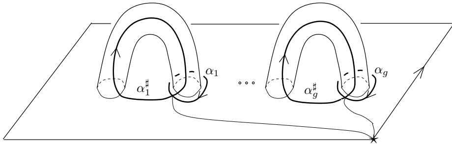
FIGURE 4.3. The surface \Sigma_{g,1} and a system of meridians and parallels (\alpha, \alpha^\#) .
