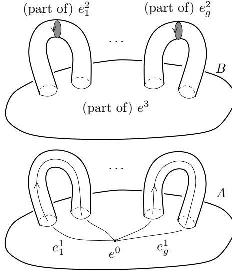
FIGURE 4.2. The cell decomposition X of M induced by the Heegaard splitting.
