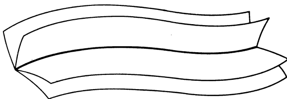
part of a \mathbb{Z}/4 -manifold
