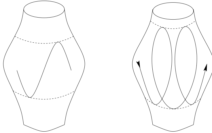
FIGURE B.1. The figure on the left-hand side shows a typical geodesic while the figure on the right-hand side shows a typical magnetic geodesic that 'curls'.
